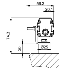
Angled fixing bracket + Antivibration support
