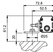
Angled fixing bracket + Orientable support
