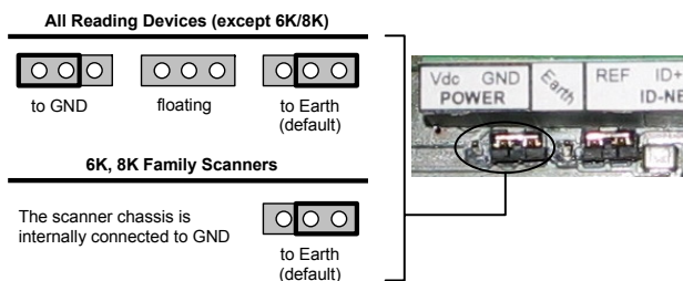
Figure 8 – Chassis Grounding
