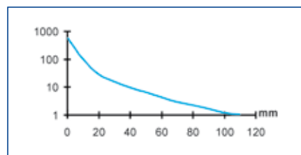
Excess gain - through beam *
