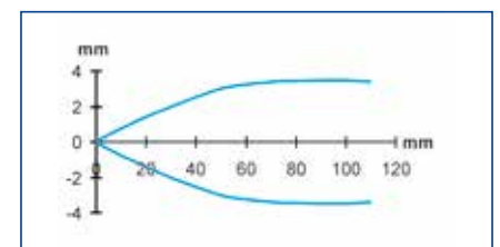
Detection area - through beam *
