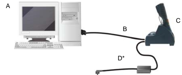
Figure 4 - RS232 Connection
