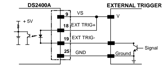
Input NPN command using DS2400A power
