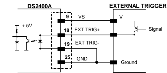
Input PNP command using DS2400A power
