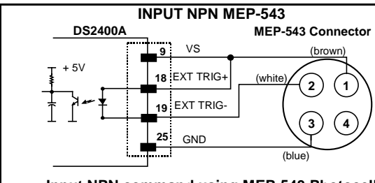
Input NPN command using MEP-543 Photocell
